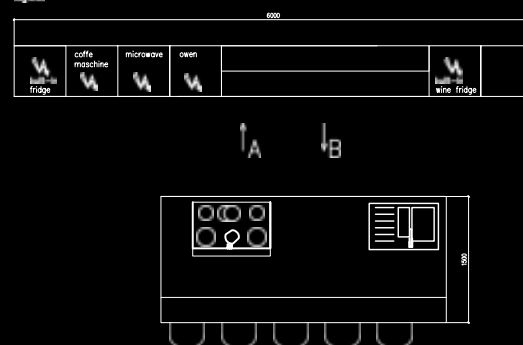
layout
