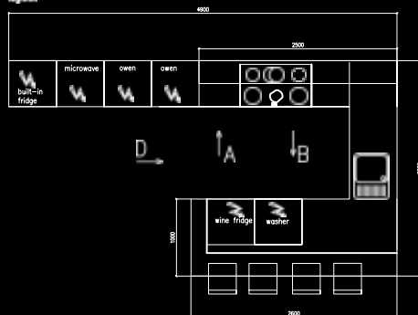
layout
