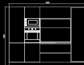
Layout
